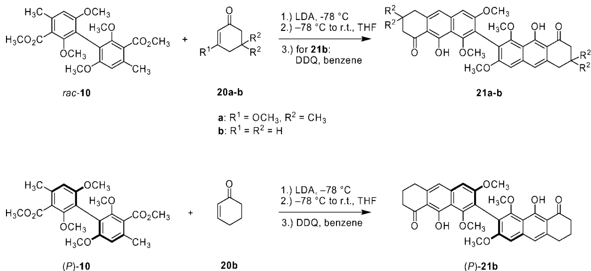
Scheme 7. Synthesis of dimeric dihydroanthracenones.
