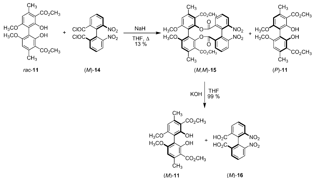
Scheme 5. Racemic resolution of dimeric orsellinate 11 by formation of diastereomeric dilactones.
