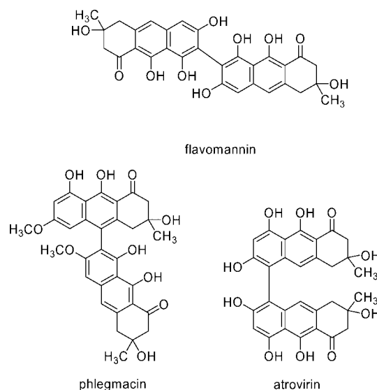
Scheme 1. Polyketide natural products containing a dimeric dihydroanthracenone structure.
