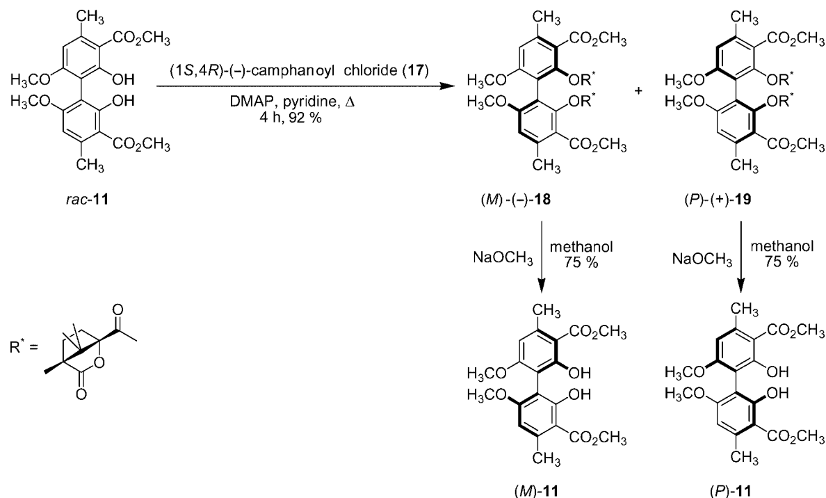
Scheme 6. Racemic resolution of dimeric orsellinate 11 by chromatographic separation of diastereomeric camphanate esters 18 and 19 .
