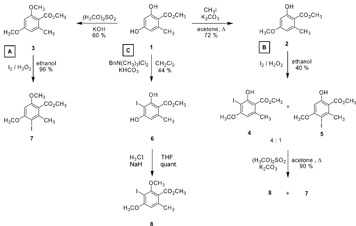
Scheme 2. Synthesis of iodinated monomeric methyl orsellinates 7 and 8 .
