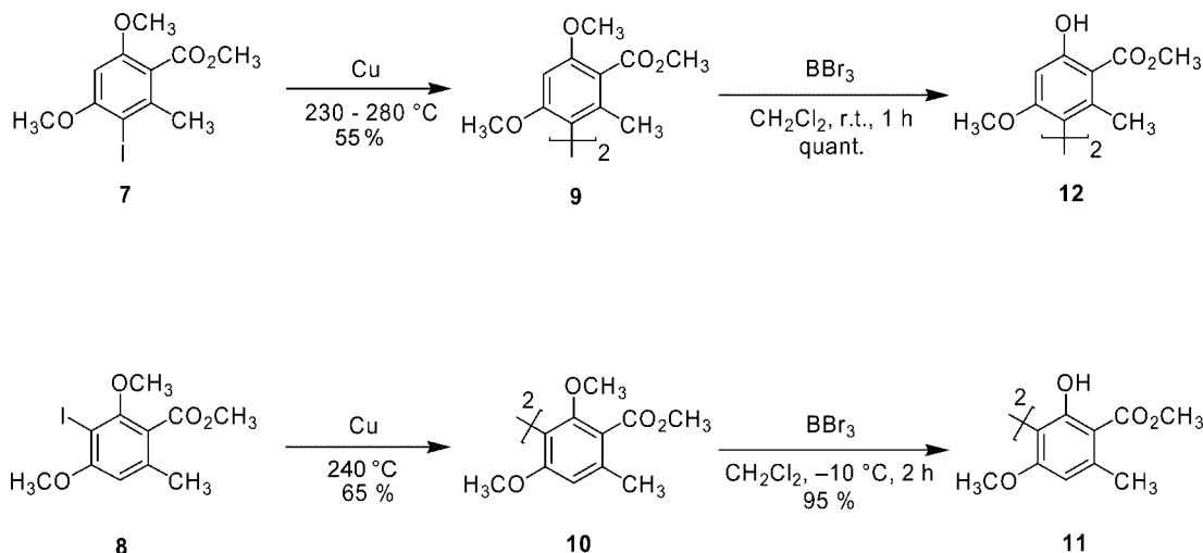
Scheme 3. Ullmann coupling of iodinated monomeric methyl orsellinates 7 and 8 , followed by selective demethylation with BBr 3 .
