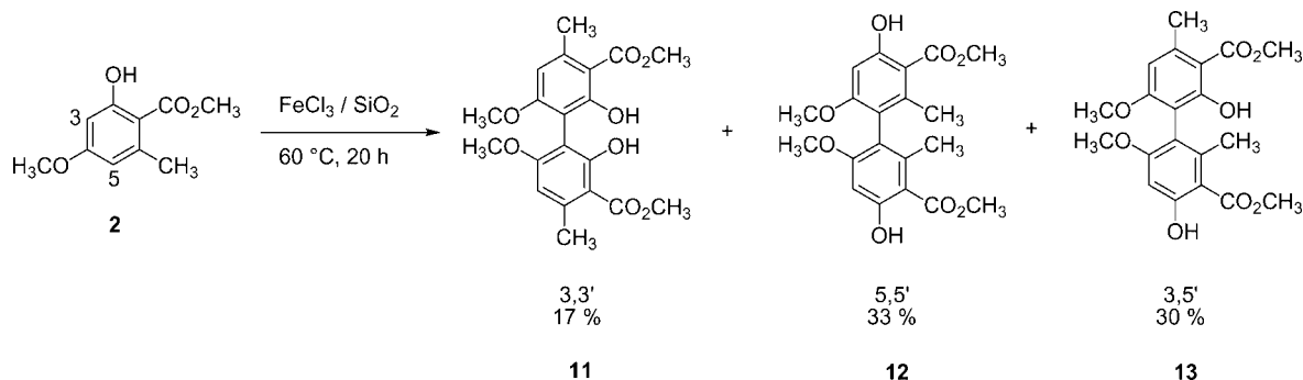
Scheme 4. Unselective oxidative phenolic coupling of 2 .
