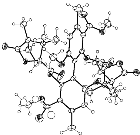
Figure 1. Molecular structure of ( M )-(–)- 18 (non-hydrogen atoms shown at 50% probability level).
